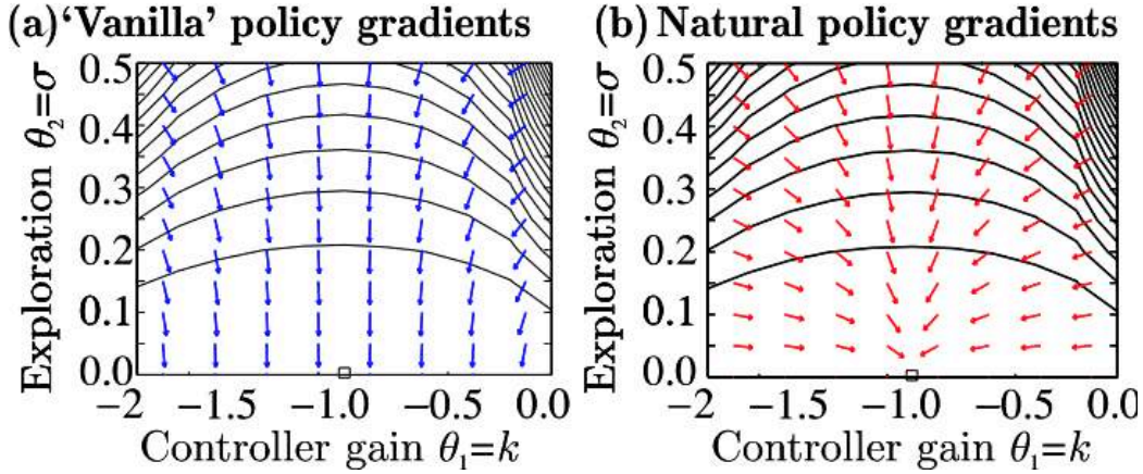
Figure 6-4. An example of the standard (left) and natural (right) policy gradients produced in a simple two-dimensional problem. Image from Peters et al. (2005) with permission.
